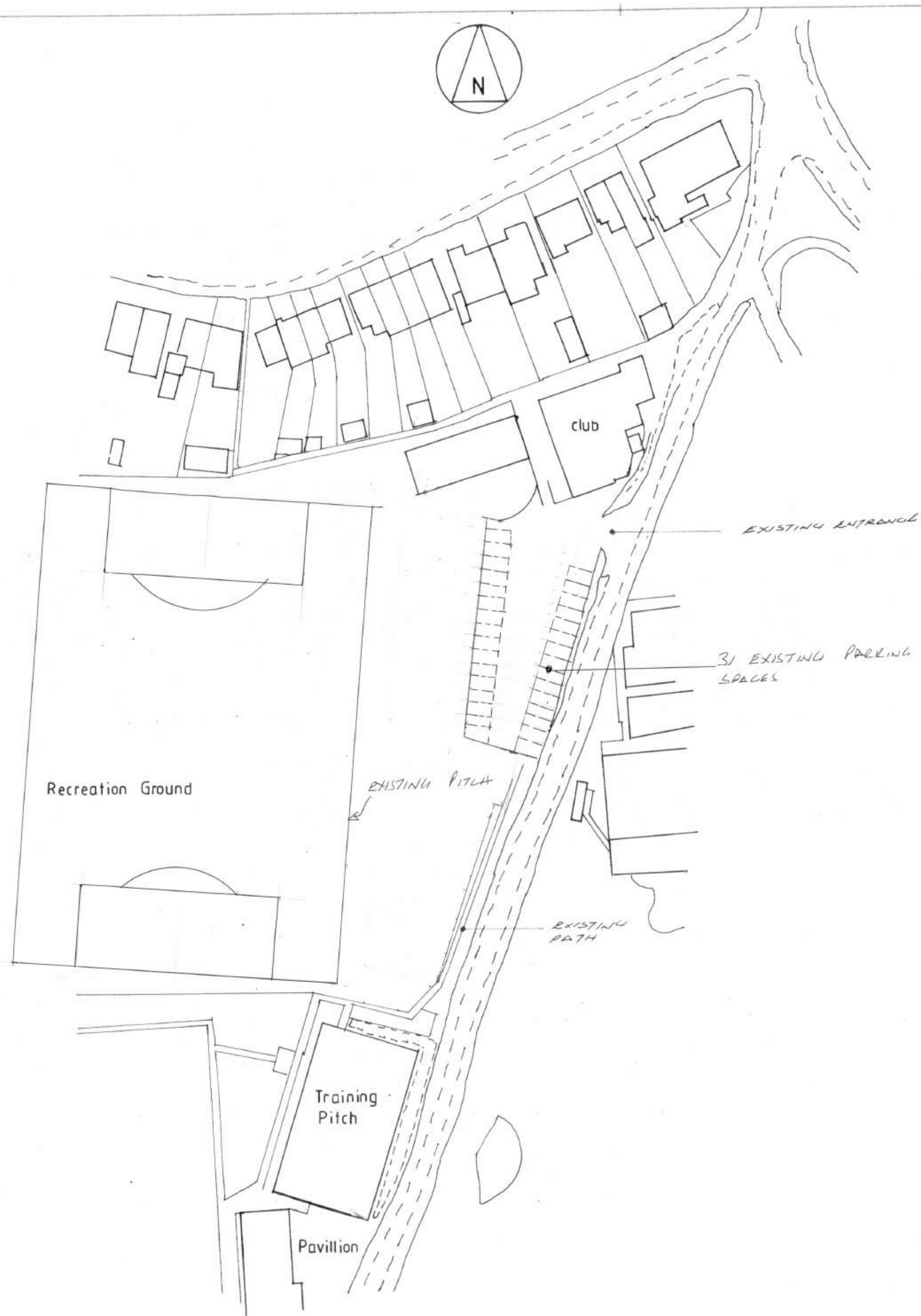
1:500 LAYOUT PLAN
