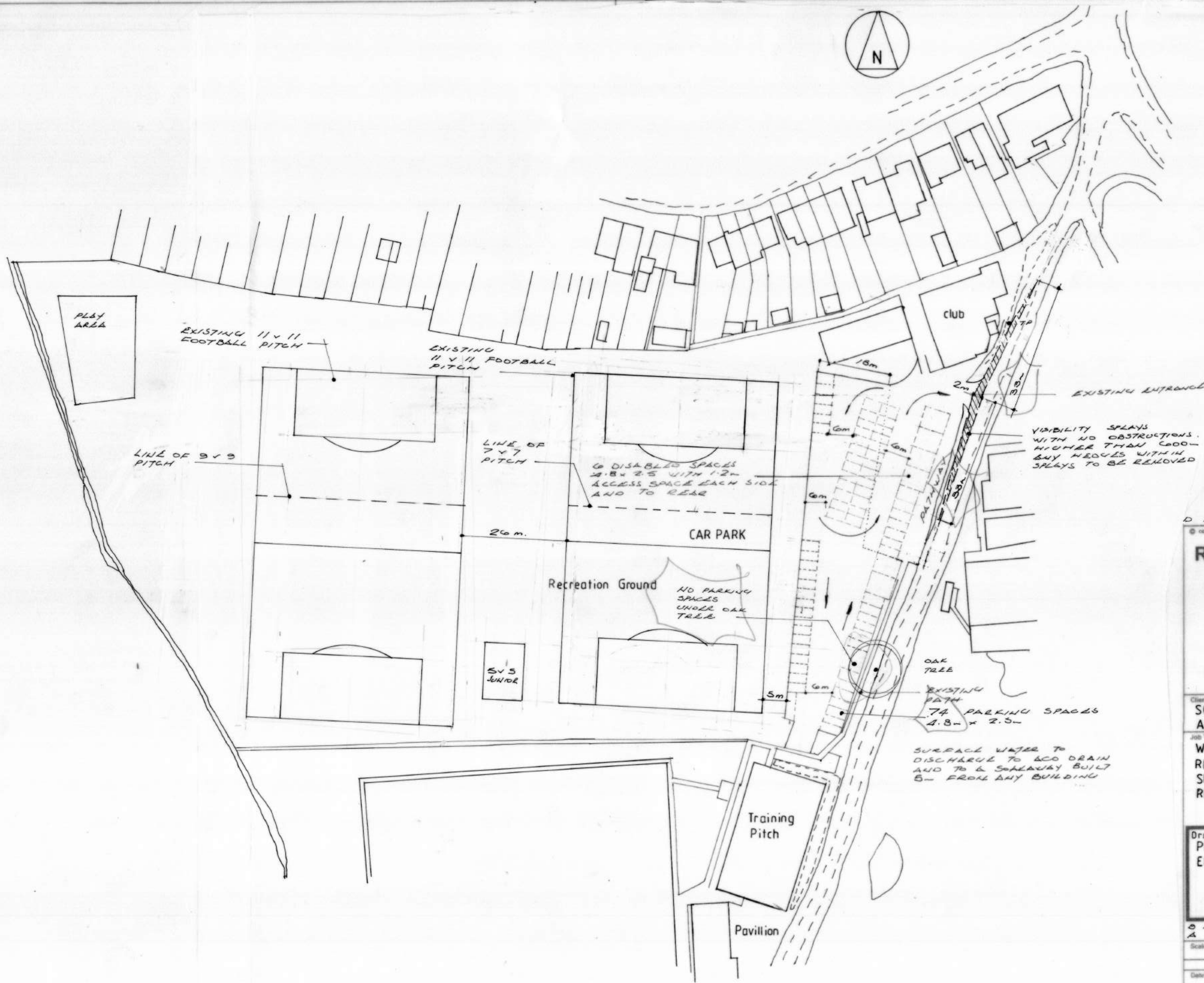
1:500 LAYOUT PLAN
